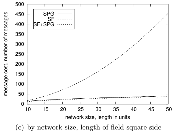
Fig. 6. Message cost normalized to geocast region size.
