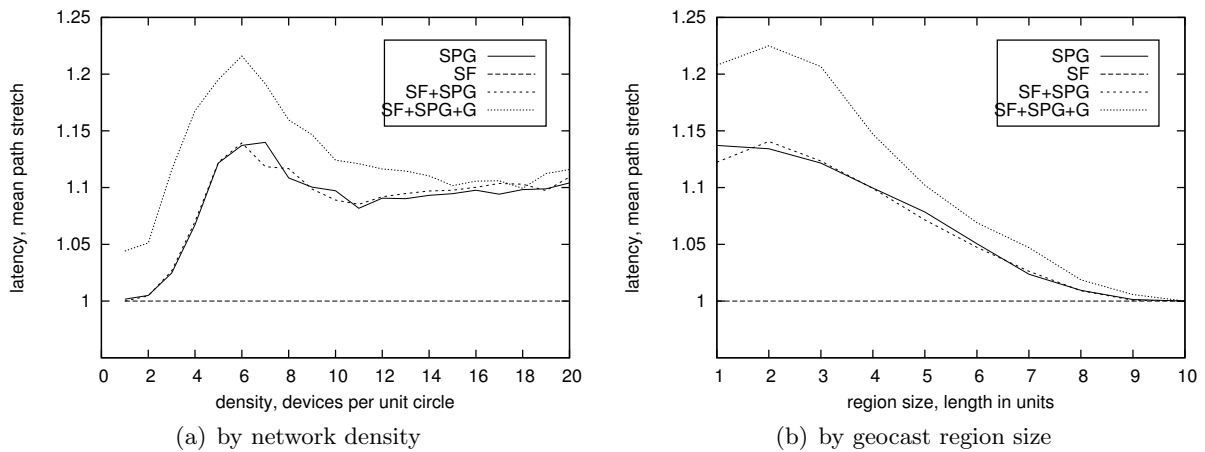
Fig. 7. Arrival latency normalized to optimal path.
